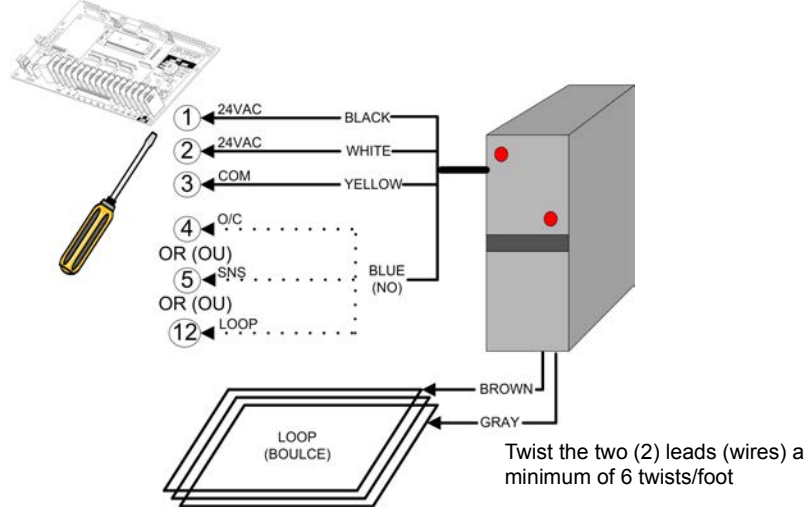
Figure 20 - Vehicle Loop Detector
