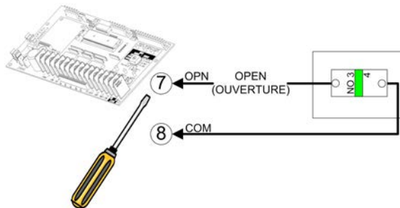
Figure 6 - STATION 001 / 081 1-PBS Open
