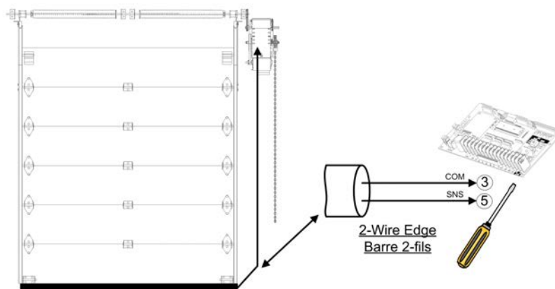
Figure 16 - Electric Reversing Edge
