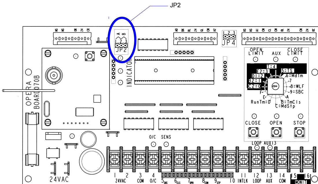
Figure 1 - Electronic Control Board – BOARD 070
