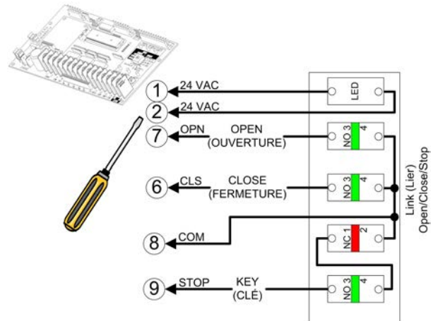
Figure 5 - STATION 080 3-PBS Open / Close / Stop with Key Lock-out and Light
