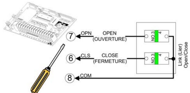
Figure 7 - STATION 010 / 082 2-PBS Open / Close
