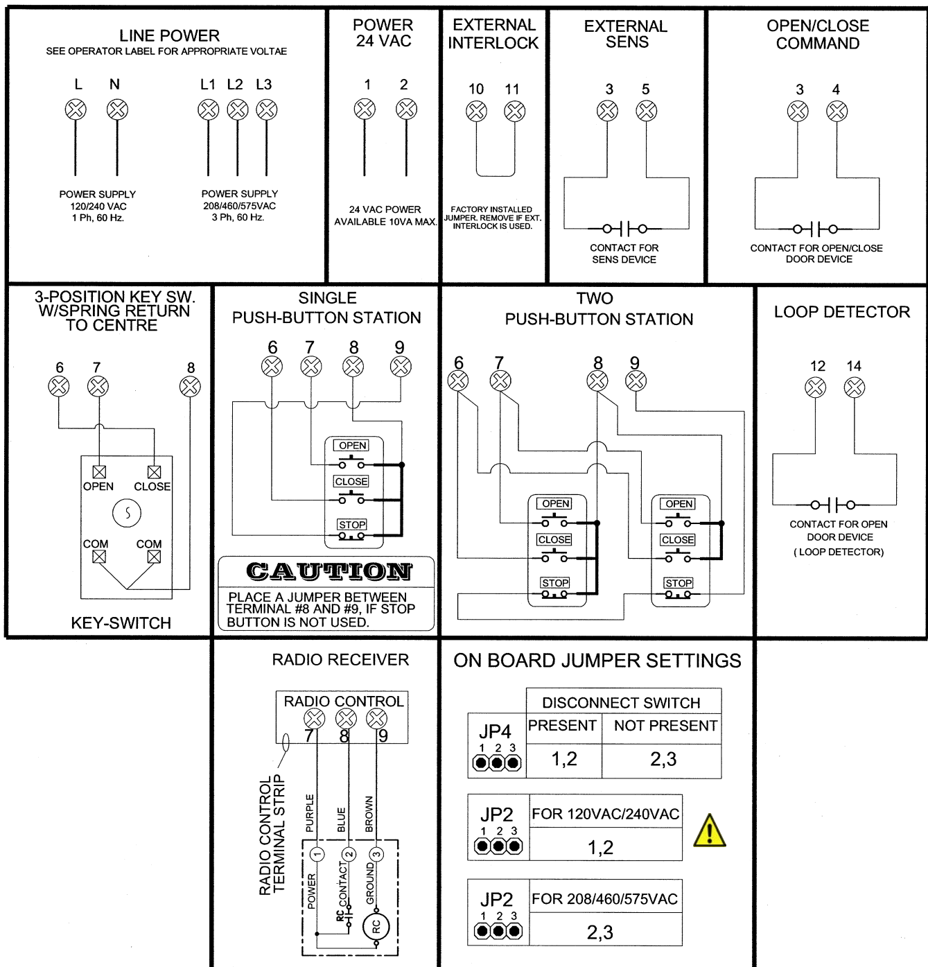
Figure 21 - External Wiring
