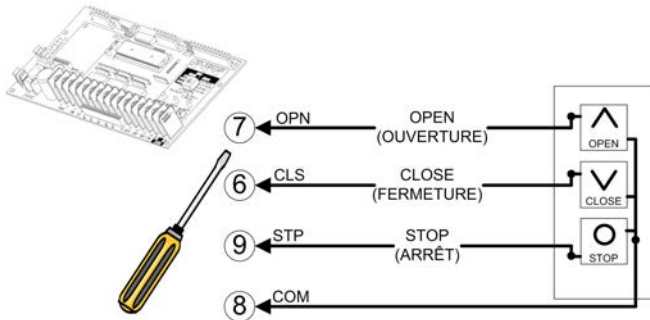
Figure 2 - STATION 020 / 084 3-PBS Open / Close / Stop
