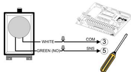
Figure 15 - AIRSWITCH 009
