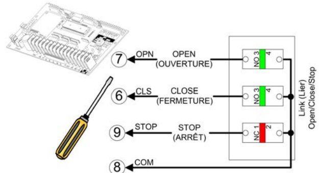
Figure 3 - STATION 041 / 049 / 056 / 076 / 078 3-PBS Open / Close / Stop
