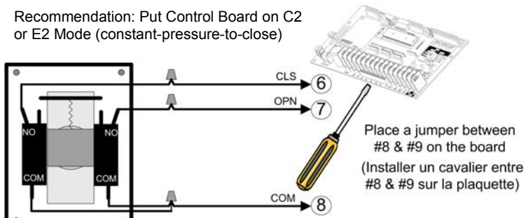
Figure 18 - KEYSWITCH 010 / 015
