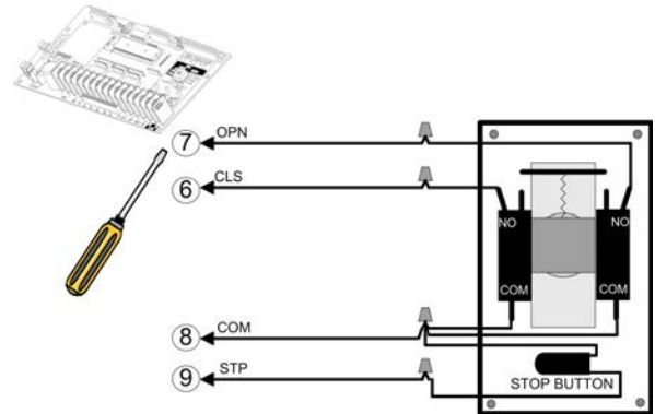
Figure 19 - KEYSWITCH 019
