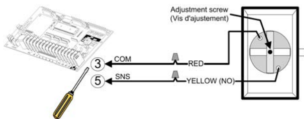
Figure 14 - AIRSWITCH 001 / 007
