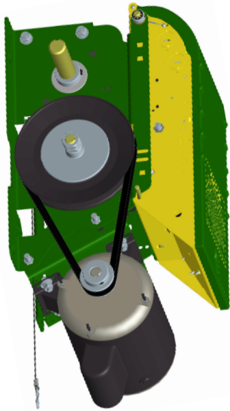
Opera-J With Solenoid Brake Installed in the Field >>>
