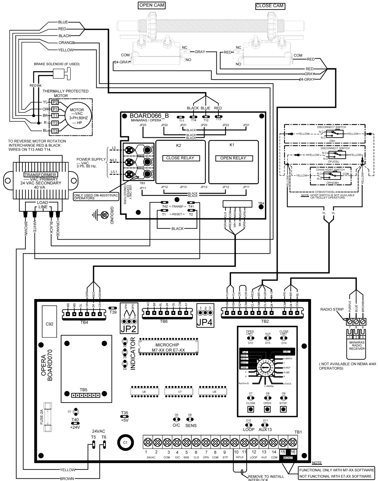
Figura 40 - EDWG1307006601
