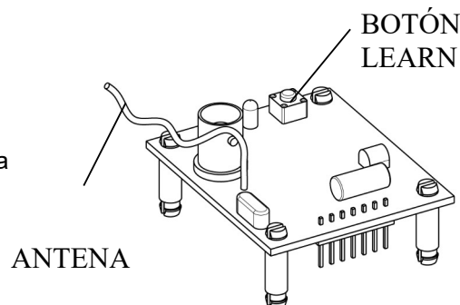
Figure 1 - RADIORE101 (ECB BOARD070)
